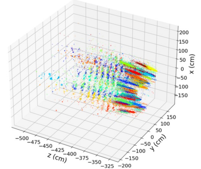
CMS Phase-2 Simulation Preliminary
